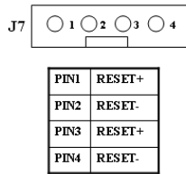
Figure2-8 Reset Pins Definitions of TD3116 Video Capture Card
