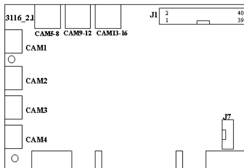
Figure2-7 TD3116 Video Capture Card
