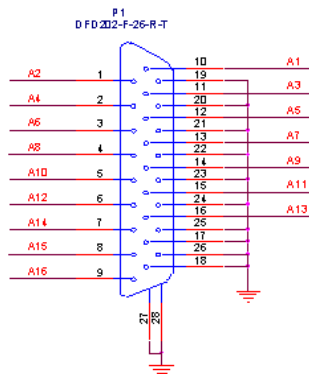
Figure2-26TD4316/4416L Video Capture Card
