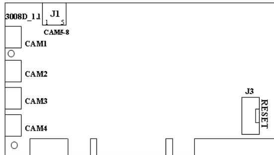
Figure2-3 TD3008 Video Capture Card
