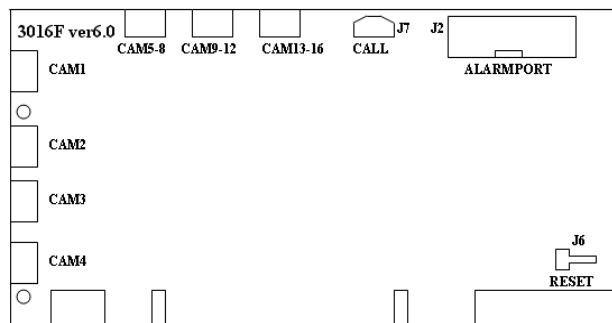
Figure2-5 TD3016 Video Capture Card Circuit Link for Watchdog Function
