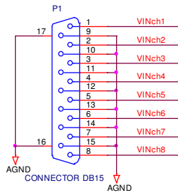
Figure2-12TD3308 Video Capture Card
