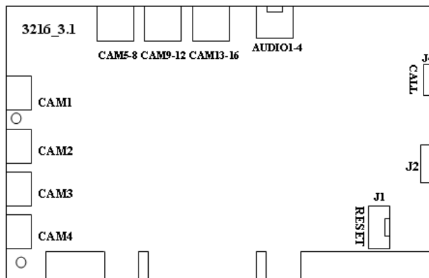
Figure2-10TD3216 Video Capture Card
