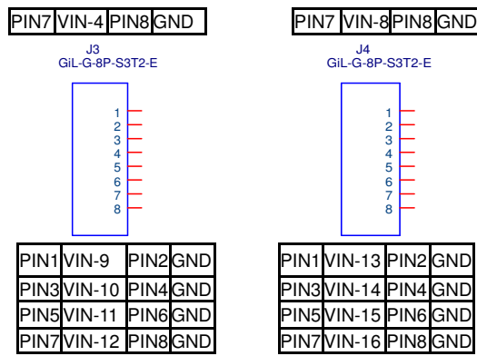
Figure2-17Video Pins Definition
