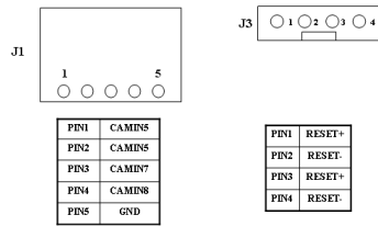
Figure2-4 Pins Definitions of TD3008 Video Capture Card
