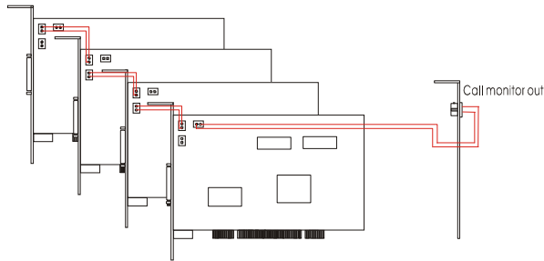
Figure2-22Multi-Card Connection
