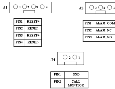
Figure2-11 Pins Definitions of TD3216 Video Capture Card
