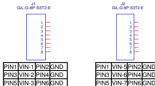
Figure2-16Audio Connector and Pins Definition
