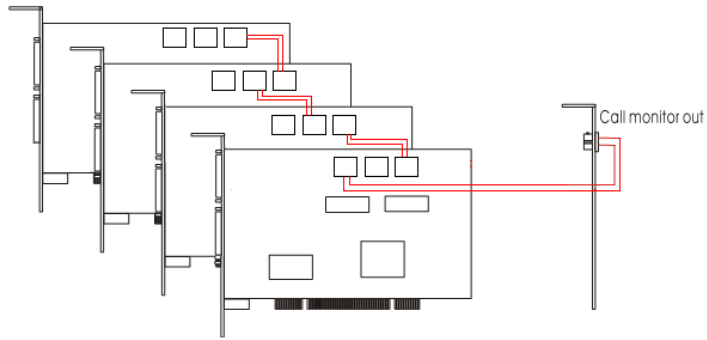
Figure2-30Multi-Card Connection
